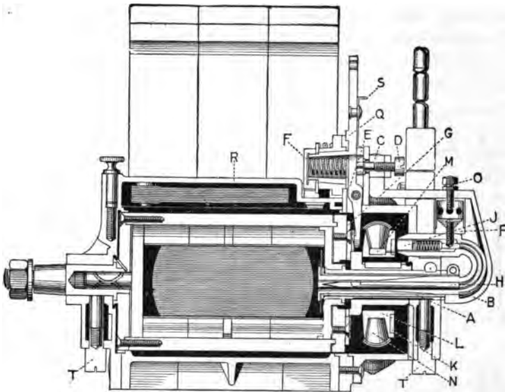
FIG. 195.—Section through the Simms-Bosch High-tension Magneto. A, armature shaft; B, curved arm carrying high tension lead; C, lug supporting screw, D, adjusting contact breaker, E, against spring, F; G, revolving sleeve carrying face cams; H, high tension lead wire; J, carbon brush of distributor disc; K, insulated ring; L, rotating drum of distributor; M and N, distributor brushes; O and O', safety spark gap; Q, swiveled lever for retarding or advancing the spark time; R, condenser; T, T, spring-pushed wick oilers for armature spindle.
